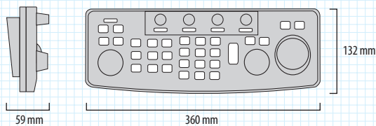
NCE-5171 Weight 1,3 kg
