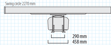
NKE-2254-9 Weight 60 kg
