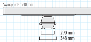
NKE-2103-6HS Weight 40 kg
